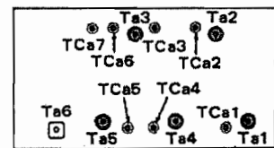
RF UNIT (X01-1220-10)
